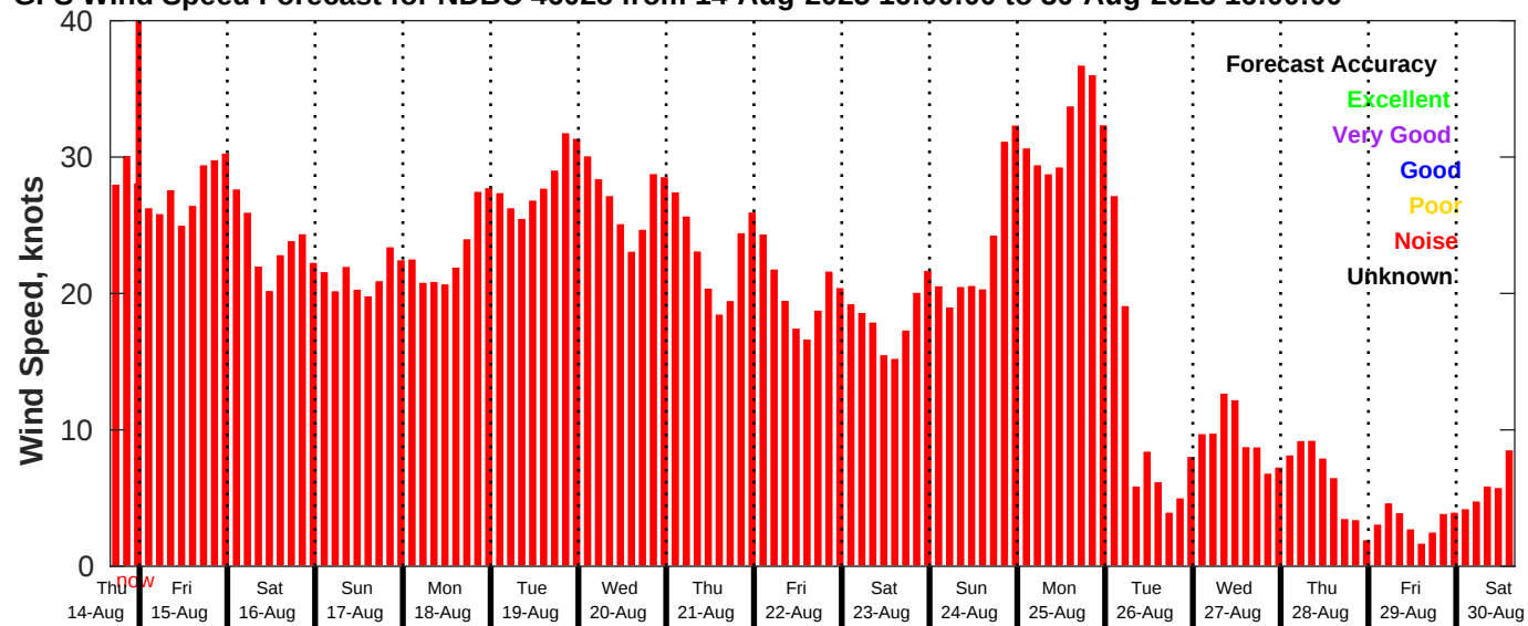
GFS Wind Speed Forecast for NDBC 46028 from 14-Aug-2025 16:00:00 to 30-Aug-2025 16:00:00
