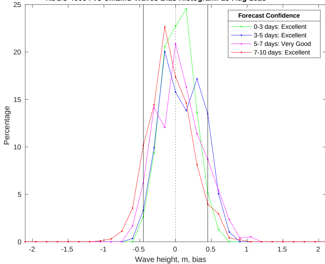
NDBC 46054 vs CMEMS Waves Bias Histogram: 15-Aug-2025
