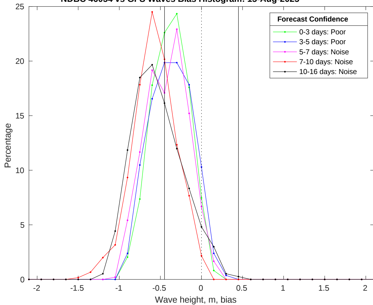
NDBC 46054 vs GFS Waves Bias Histogram: 15-Aug-2025
