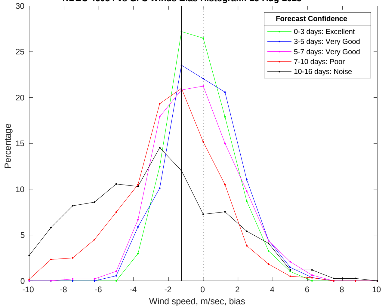
NDBC 46054 vs GFS Winds Bias Histogram: 15-Aug-2025
