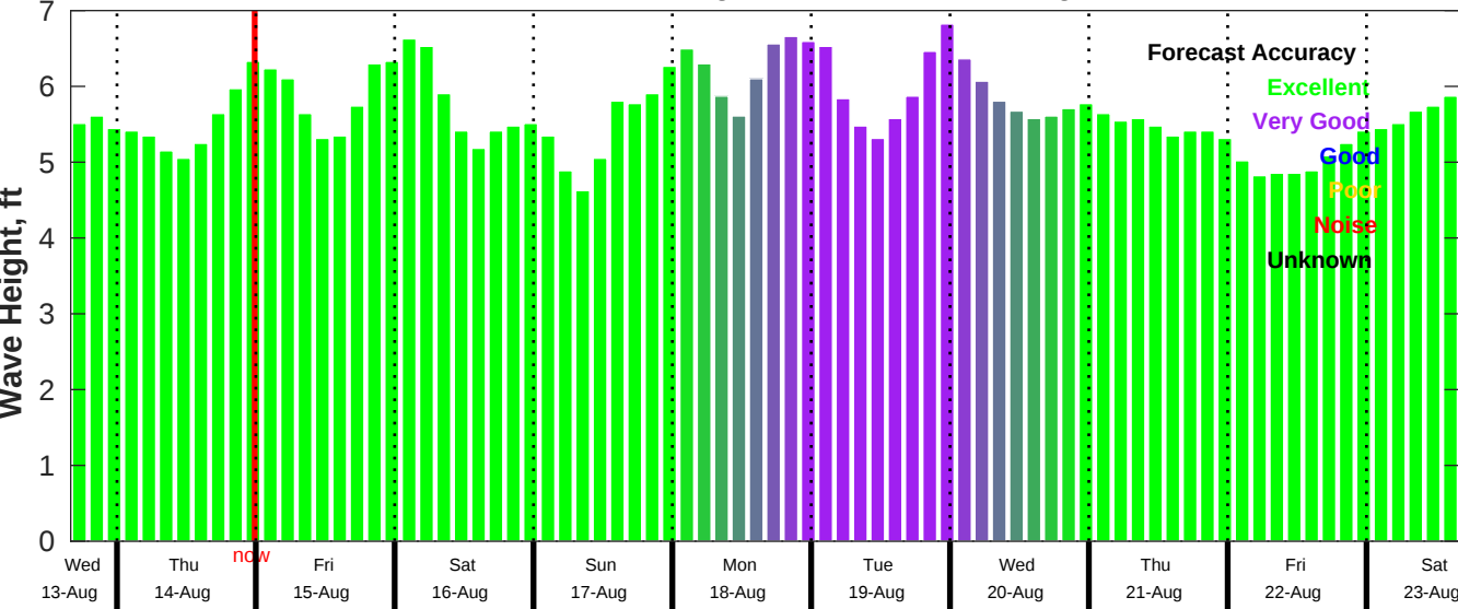
CMEMS Wave Forecast for NDBC 46054 from 13-Aug-2025 16:00:00 to 23-Aug-2025 16:00:00
