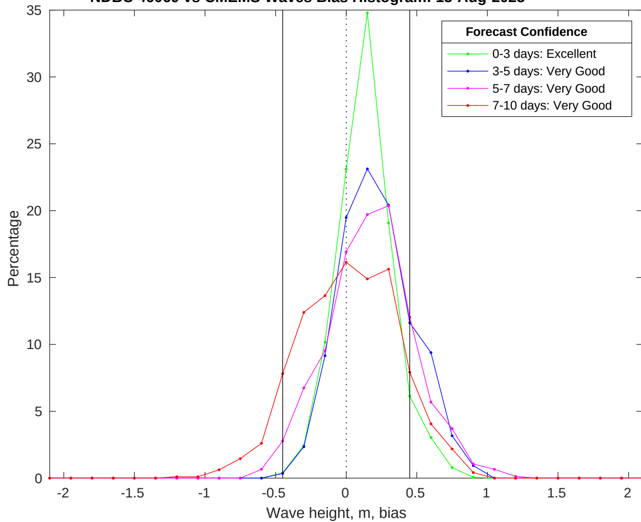
NDBC 46069 vs CMEMS Waves Bias Histogram: 15-Aug-2025
