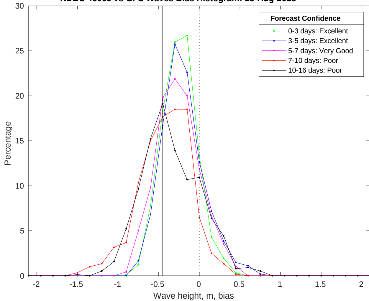
NDBC 46069 vs GFS Waves Bias Histogram: 15-Aug-2025
