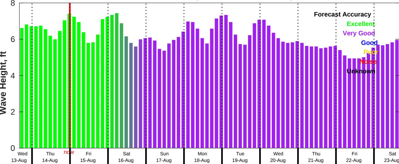
CMEMS Wave Forecast for NDBC 46069 from 13-Aug-2025 16:00:00 to 23-Aug-2025 16:00:00
