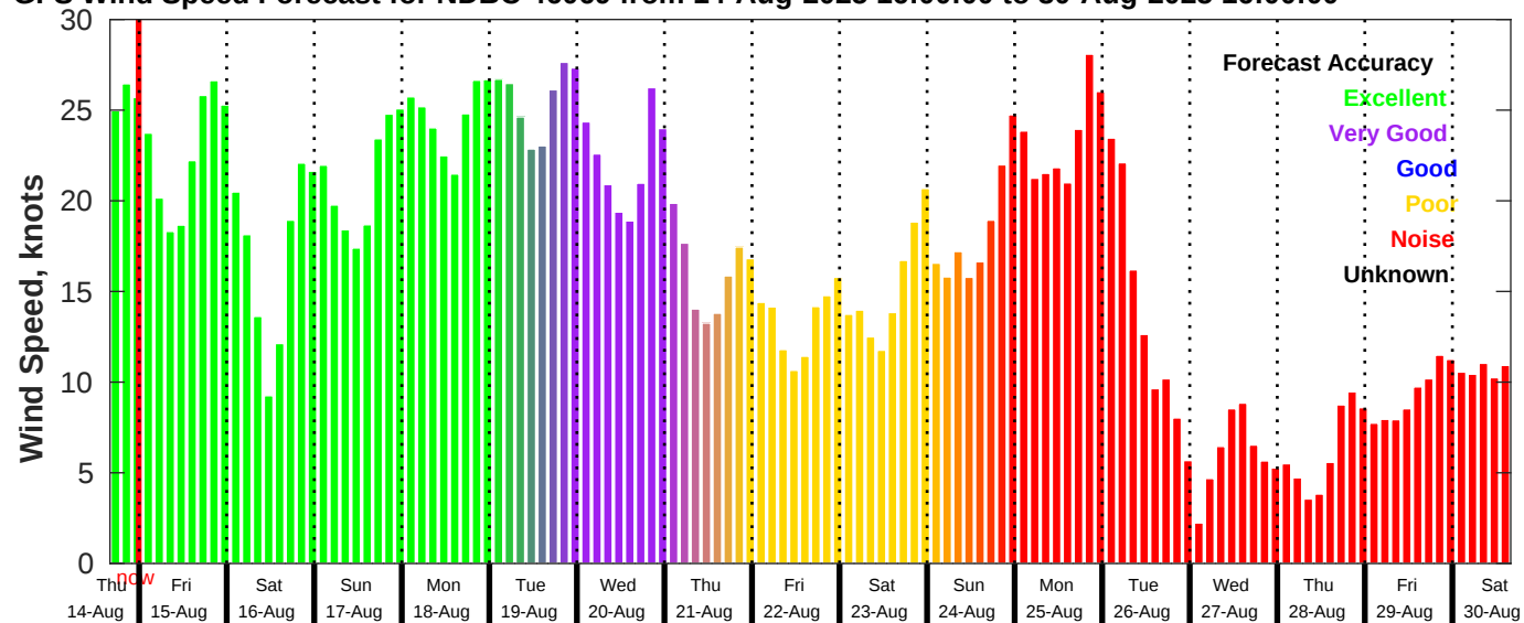
GFS Wind Speed Forecast for NDBC 46069 from 14-Aug-2025 16:00:00 to 30-Aug-2025 16:00:00
