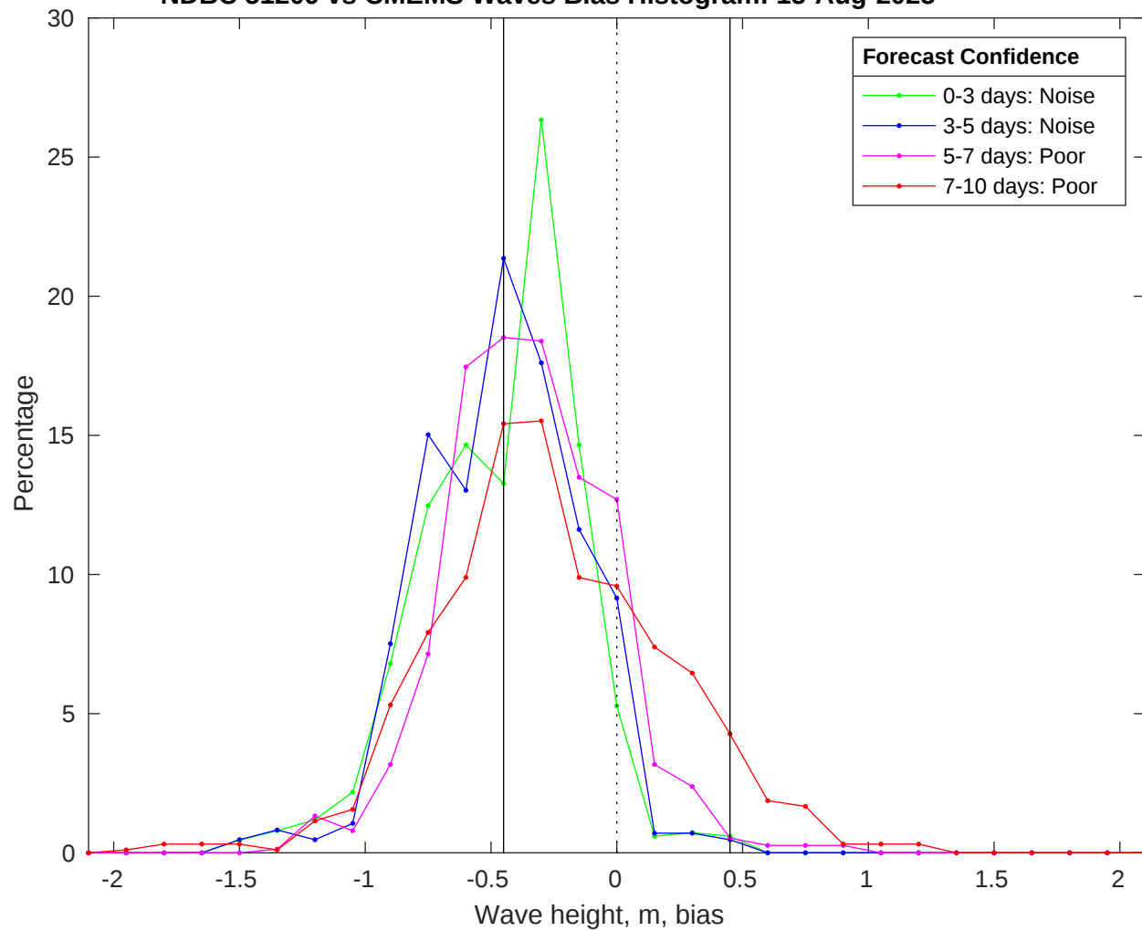
NDBC 51209 vs CMEMS Waves Bias Histogram: 15-Aug-2025
