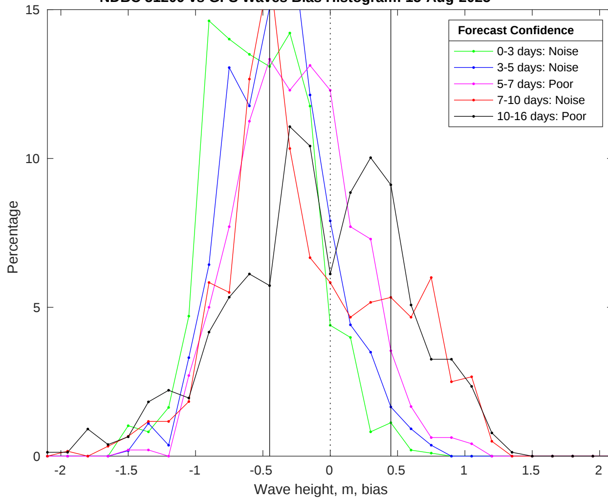
NDBC 51209 vs GFS Waves Bias Histogram: 15-Aug-2025
