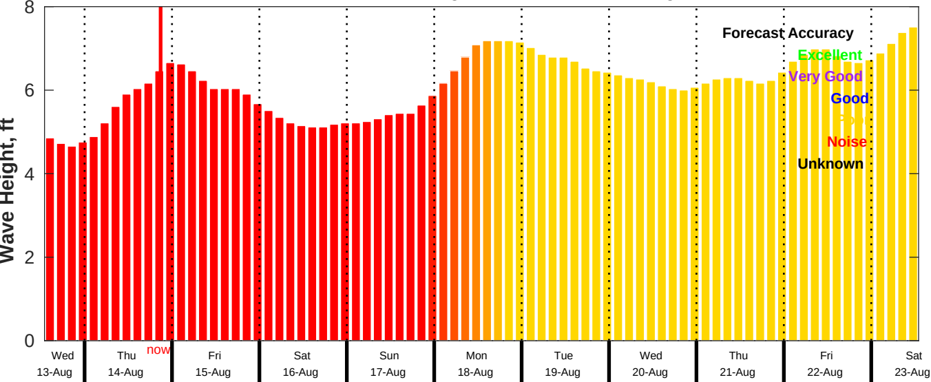
CMEMS Wave Forecast for NDBC 51209 from 13-Aug-2025 13:00:00 to 23-Aug-2025 13:00:00
