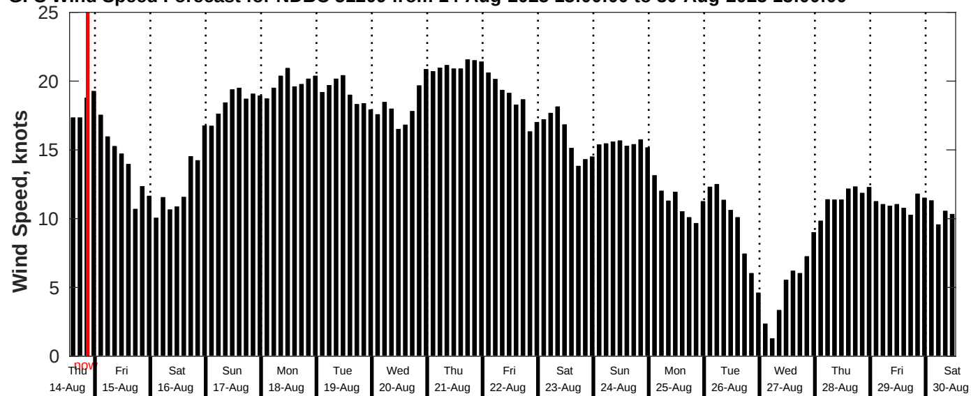
GFS Wind Speed Forecast for NDBC 51209 from 14-Aug-2025 13:00:00 to 30-Aug-2025 13:00:00
