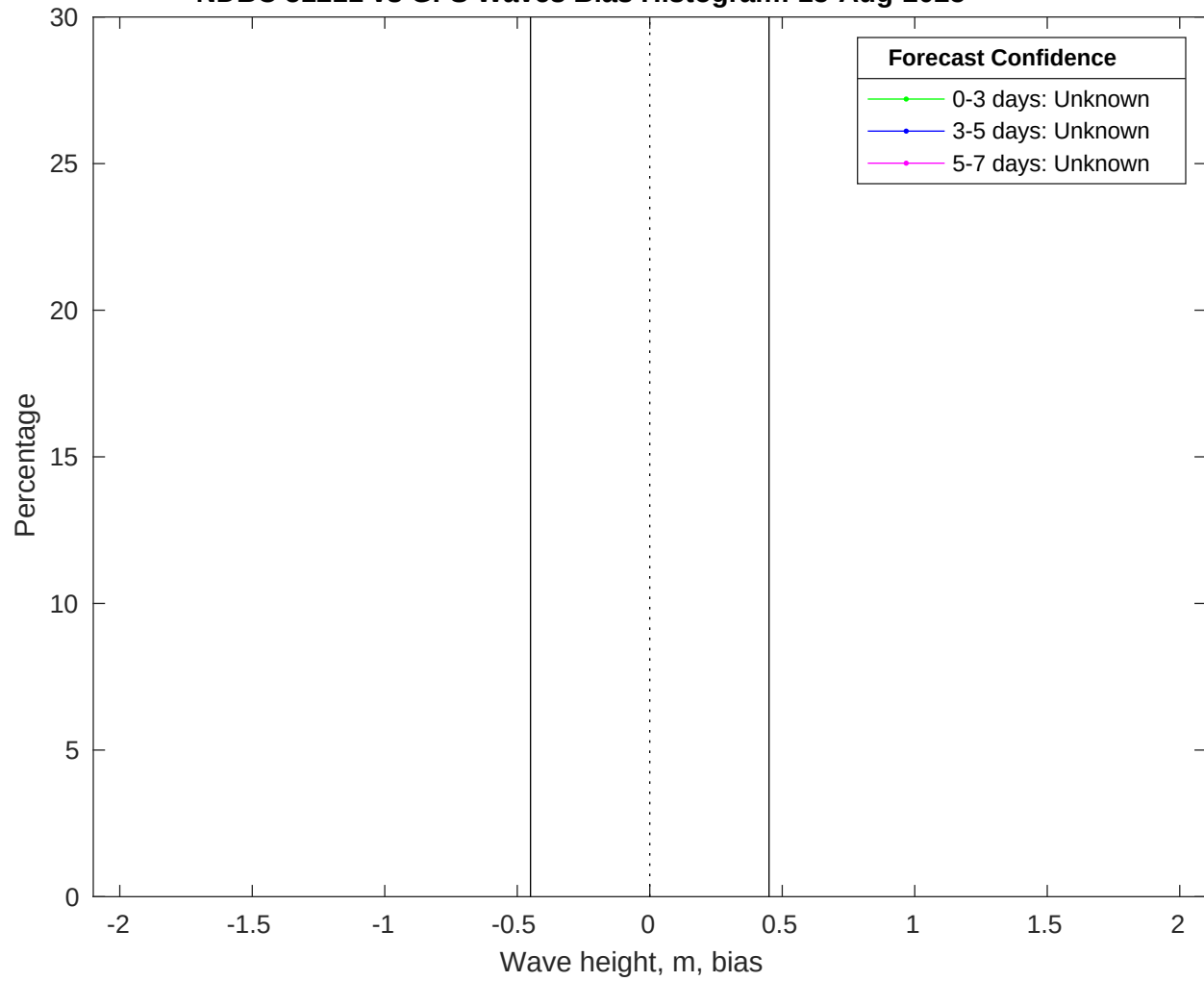
NDBC 51211 vs GFS Waves Bias Histogram: 15-Aug-2025
