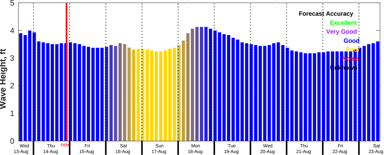
CMEMS Wave Forecast for NDBC 51211 from 13-Aug-2025 14:00:00 to 23-Aug-2025 14:00:00
