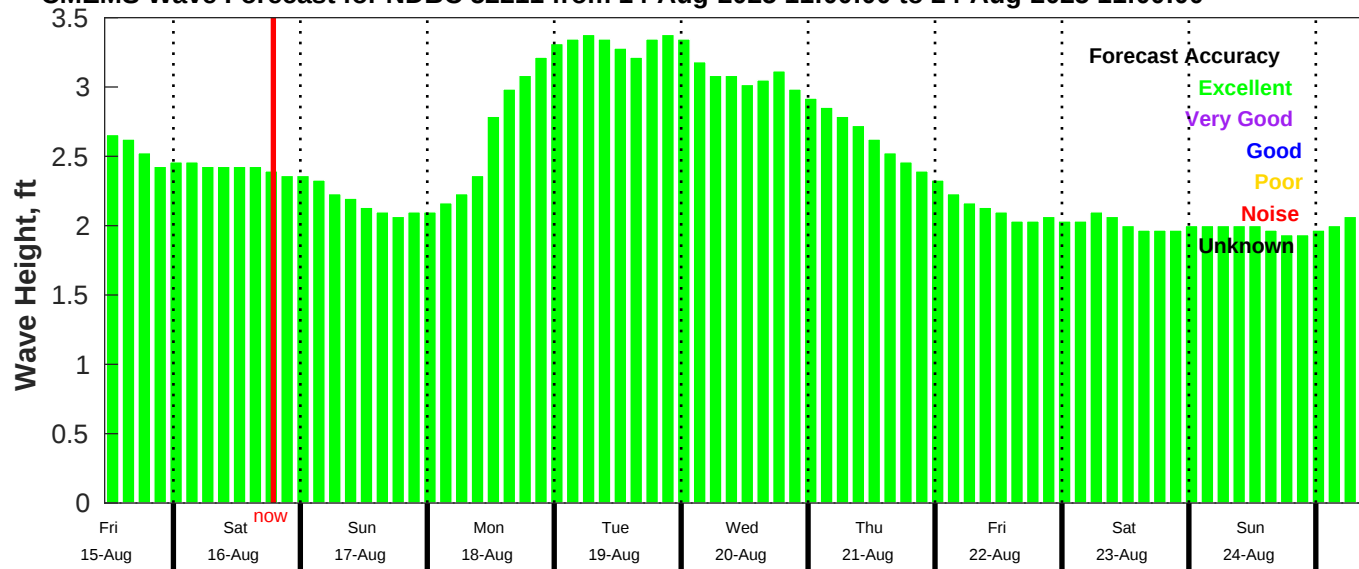
CMEMS Wave Forecast for NDBC 52211 from 14-Aug-2025 11:00:00 to 24-Aug-2025 11:00:00
