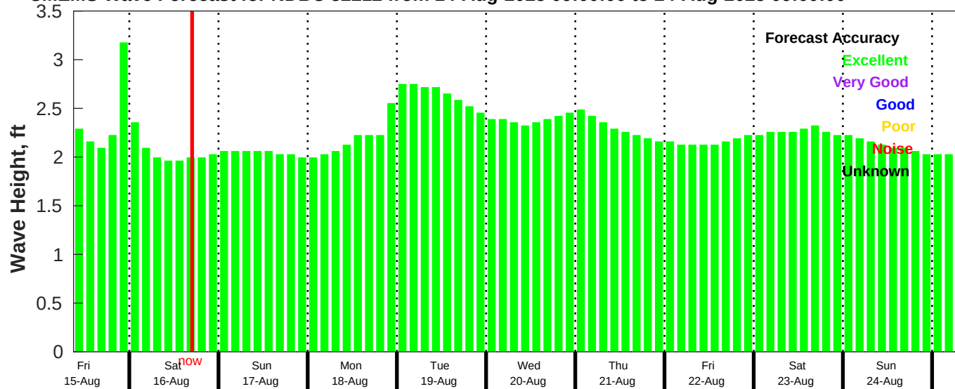
CMEMS Wave Forecast for NDBC 52212 from 14-Aug-2025 09:00:00 to 24-Aug-2025 09:00:00
