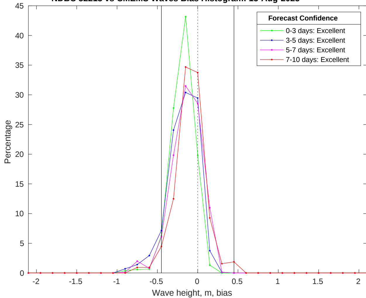
NDBC 52213 vs CMEMS Waves Bias Histogram: 15-Aug-2025
