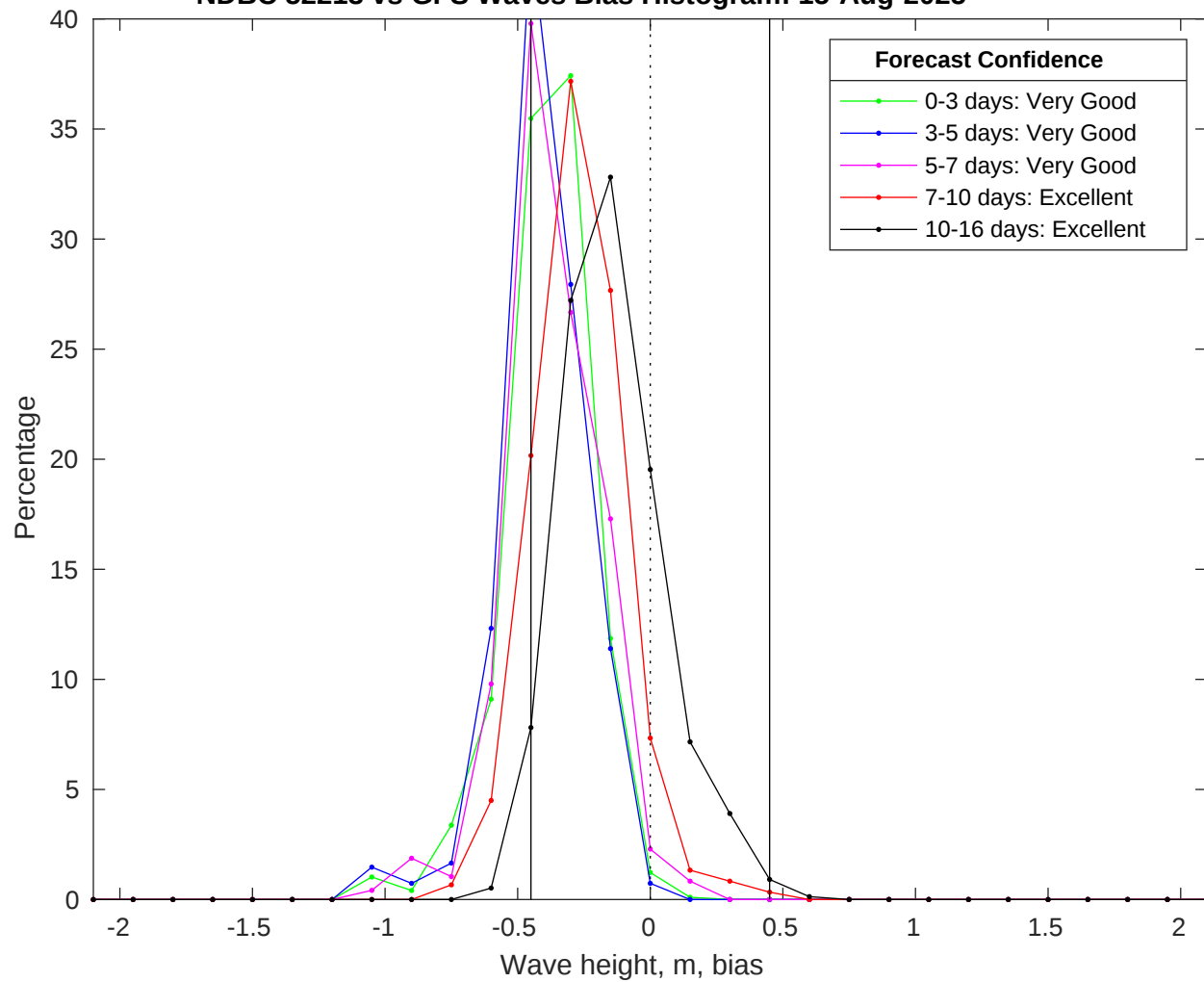
NDBC 52213 vs GFS Waves Bias Histogram: 15-Aug-2025
