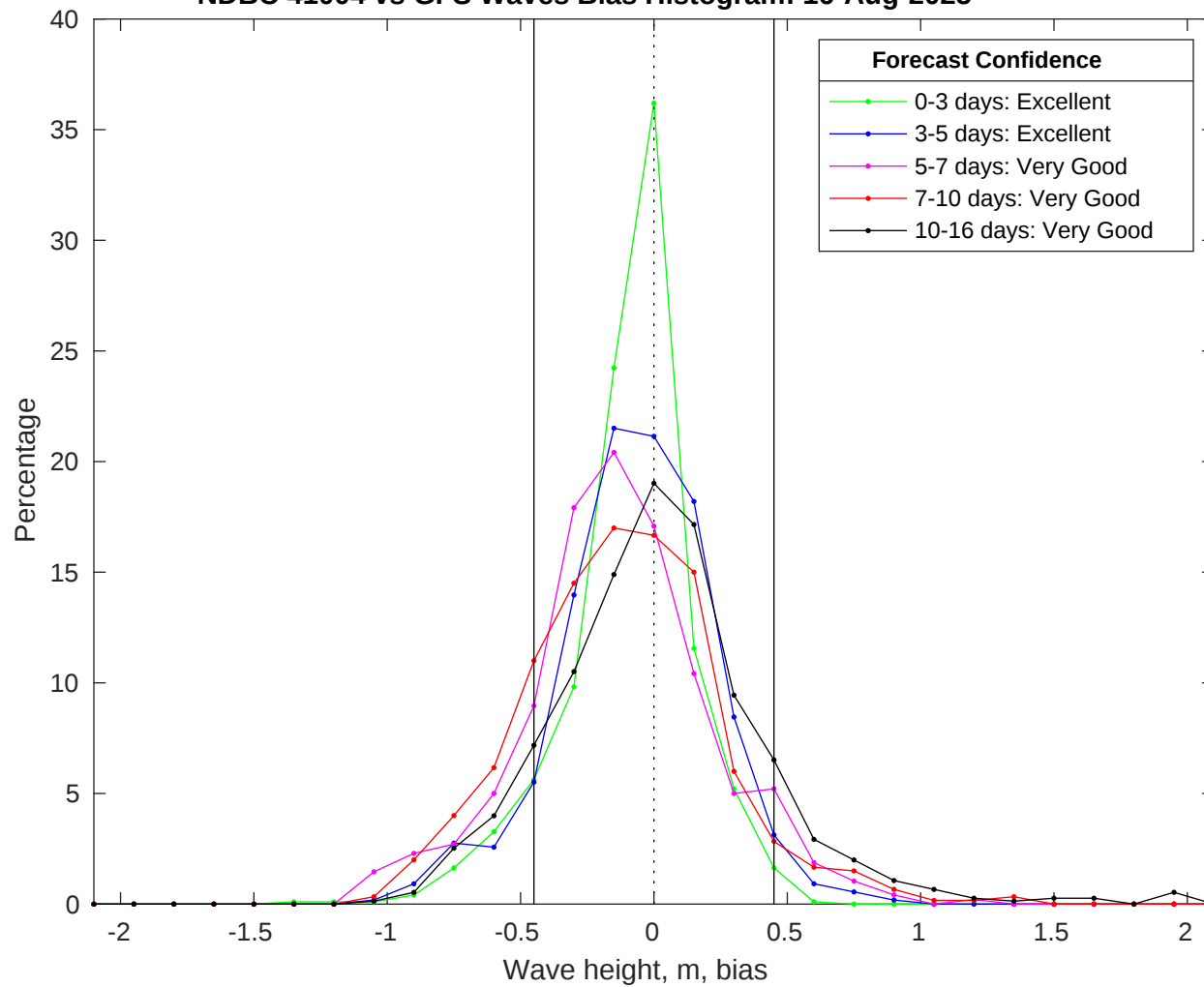
NDBC 41004 vs GFS Waves Bias Histogram: 16-Aug-2025
