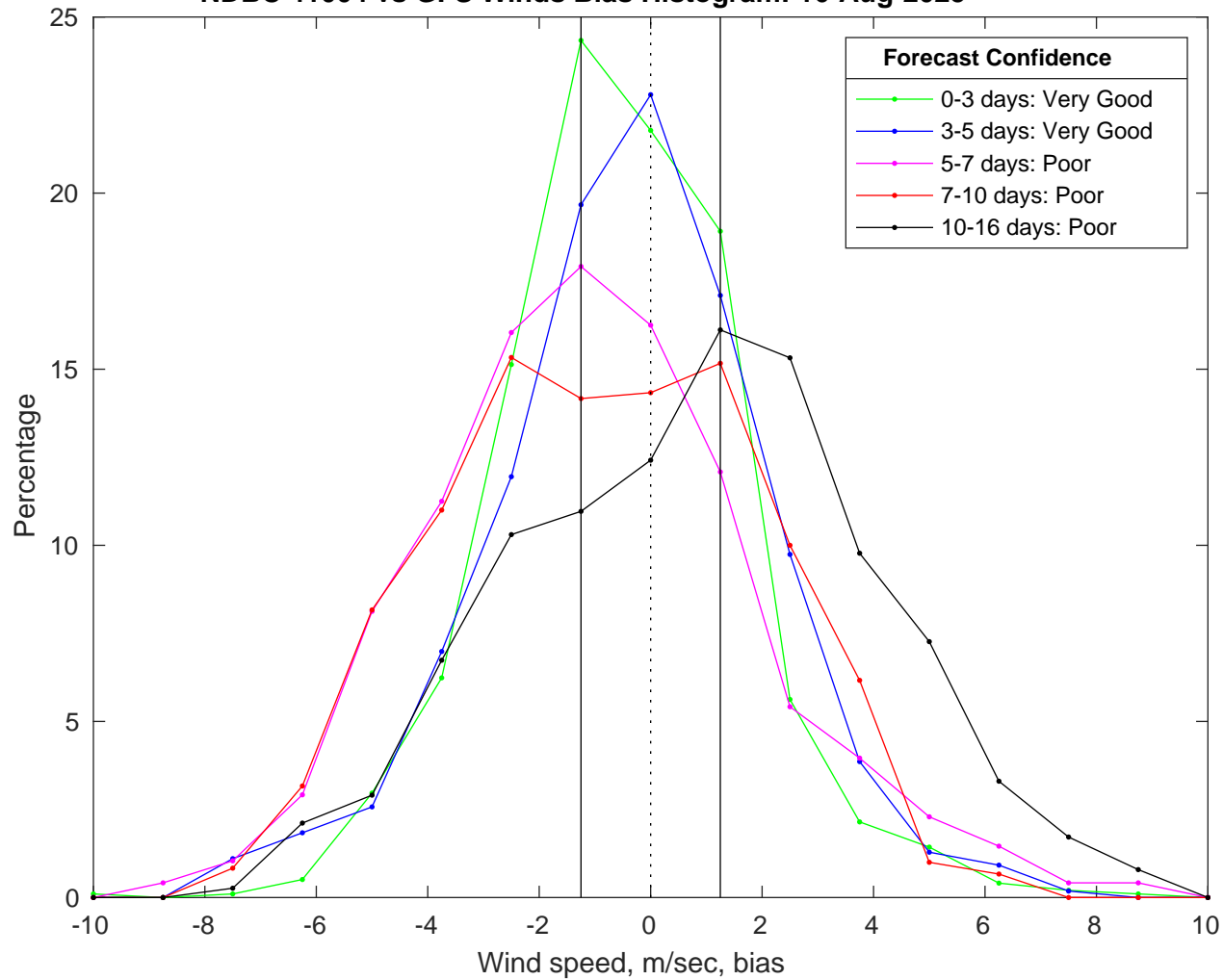
NDBC 41004 vs GFS Winds Bias Histogram: 16-Aug-2025
