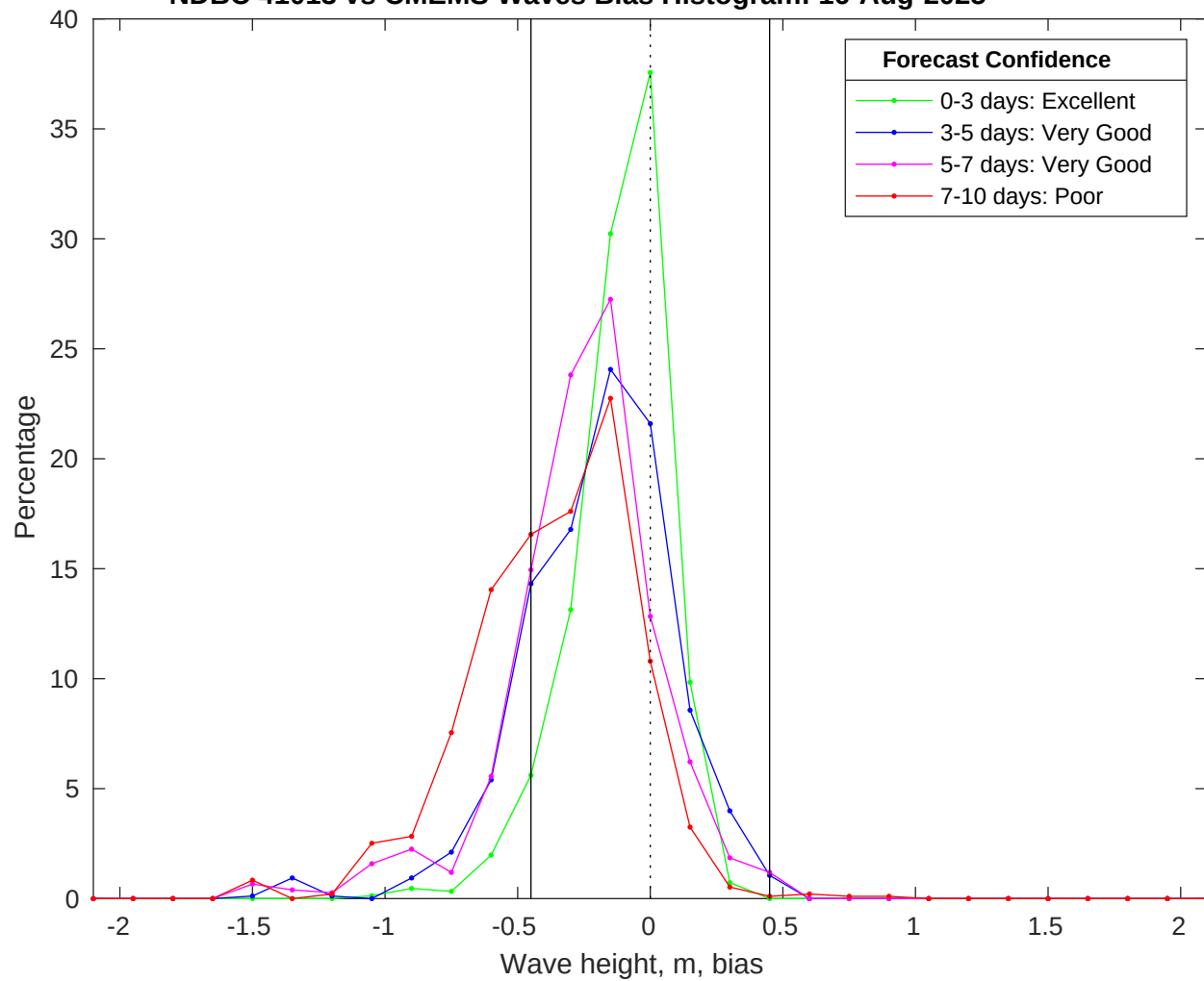
NDBC 41013 vs CMEMS Waves Bias Histogram: 16-Aug-2025
