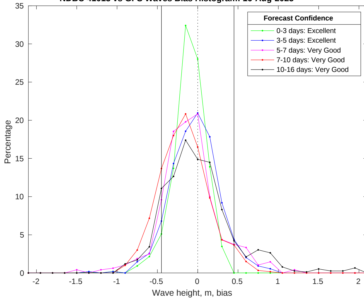
NDBC 41013 vs GFS Waves Bias Histogram: 16-Aug-2025
