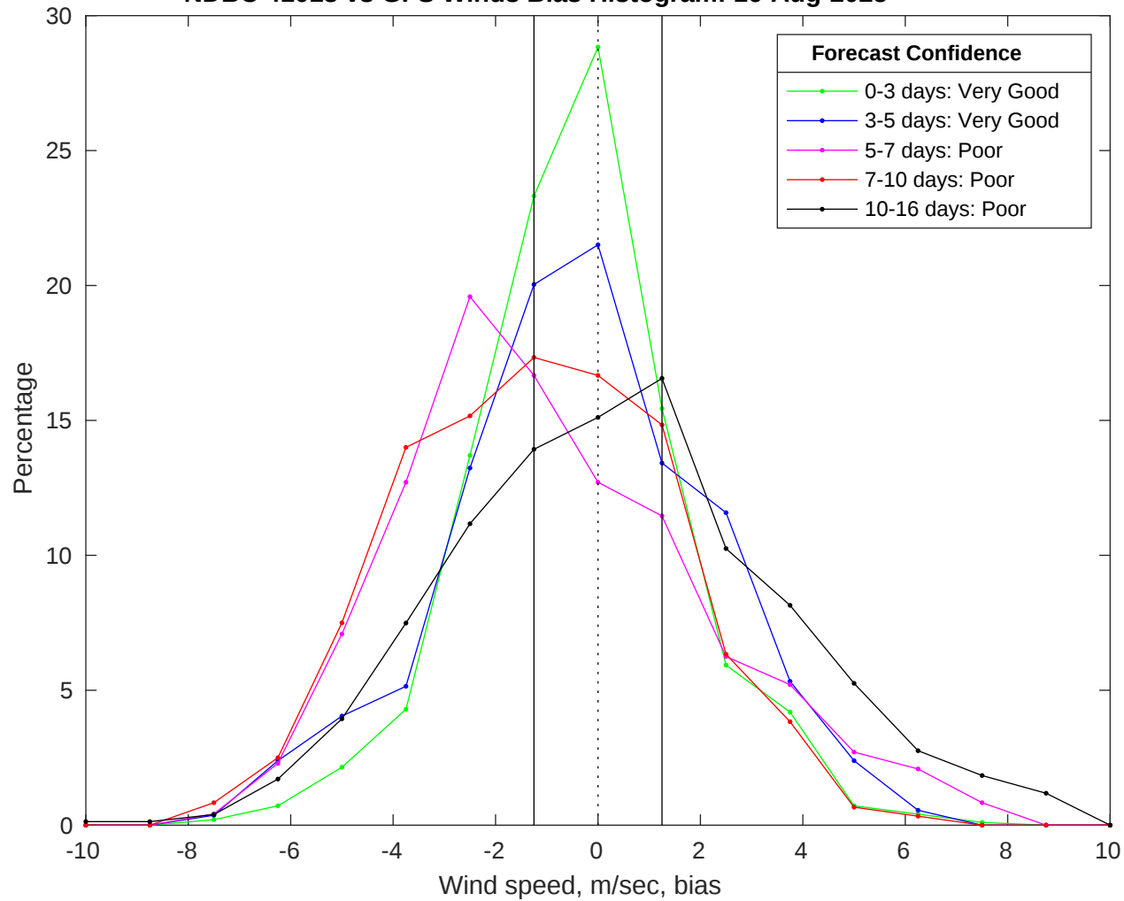
NDBC 41013 vs GFS Winds Bias Histogram: 16-Aug-2025
