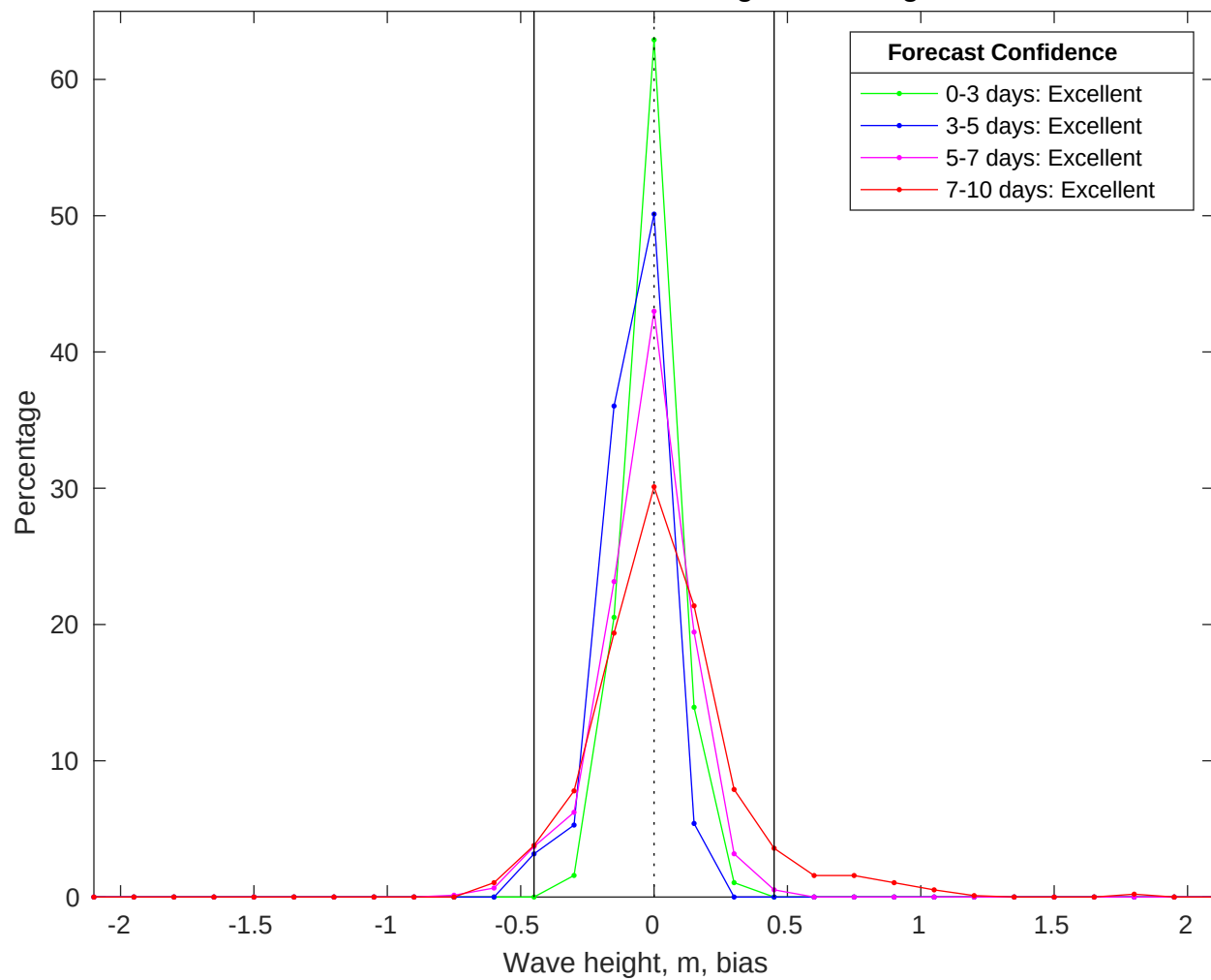
NDBC 41040 vs CMEMS Waves Bias Histogram: 16-Aug-2025
