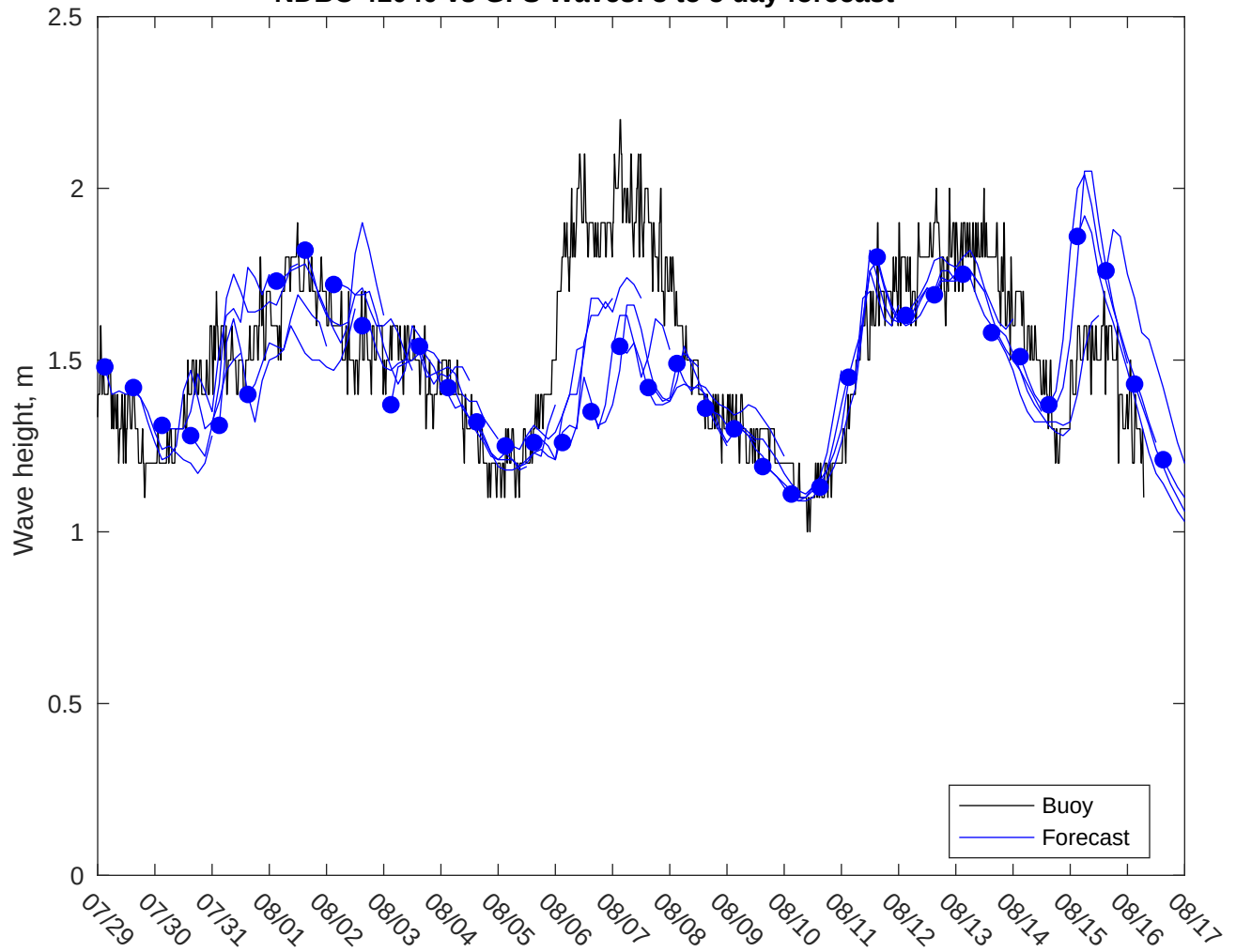
NDBC 41040 vs GFS Waves: 3 to 5 day forecast
