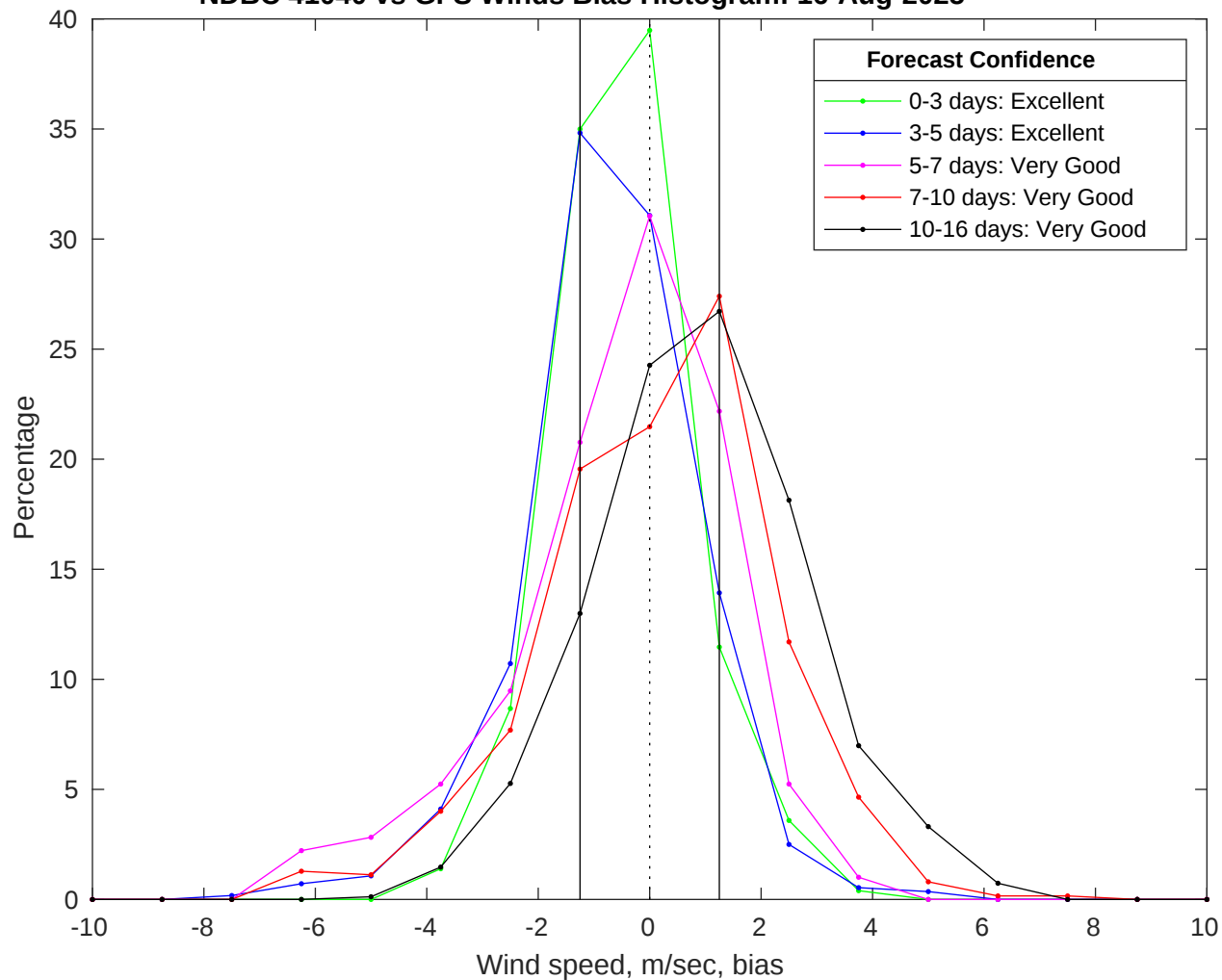
NDBC 41040 vs GFS Winds Bias Histogram: 16-Aug-2025
