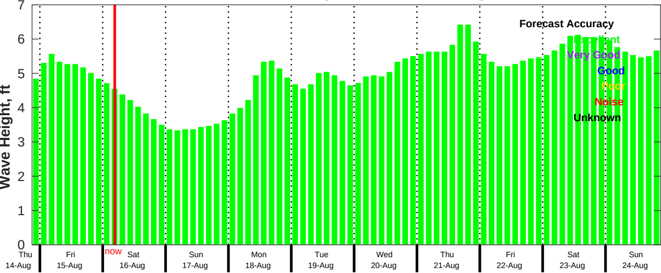
CMEMS Wave Forecast for NDBC 41040 from 14-Aug-2025 21:00:00 to 24-Aug-2025 21:00:00
