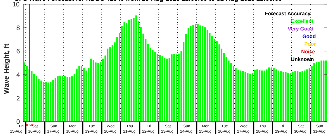
GFS Wave Forecast for NDBC 41040 from 15-Aug-2025 21:00:00 to 31-Aug-2025 21:00:00
