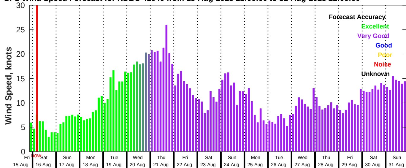
GFS Wind Speed Forecast for NDBC 41040 from 15-Aug-2025 21:00:00 to 31-Aug-2025 21:00:00
