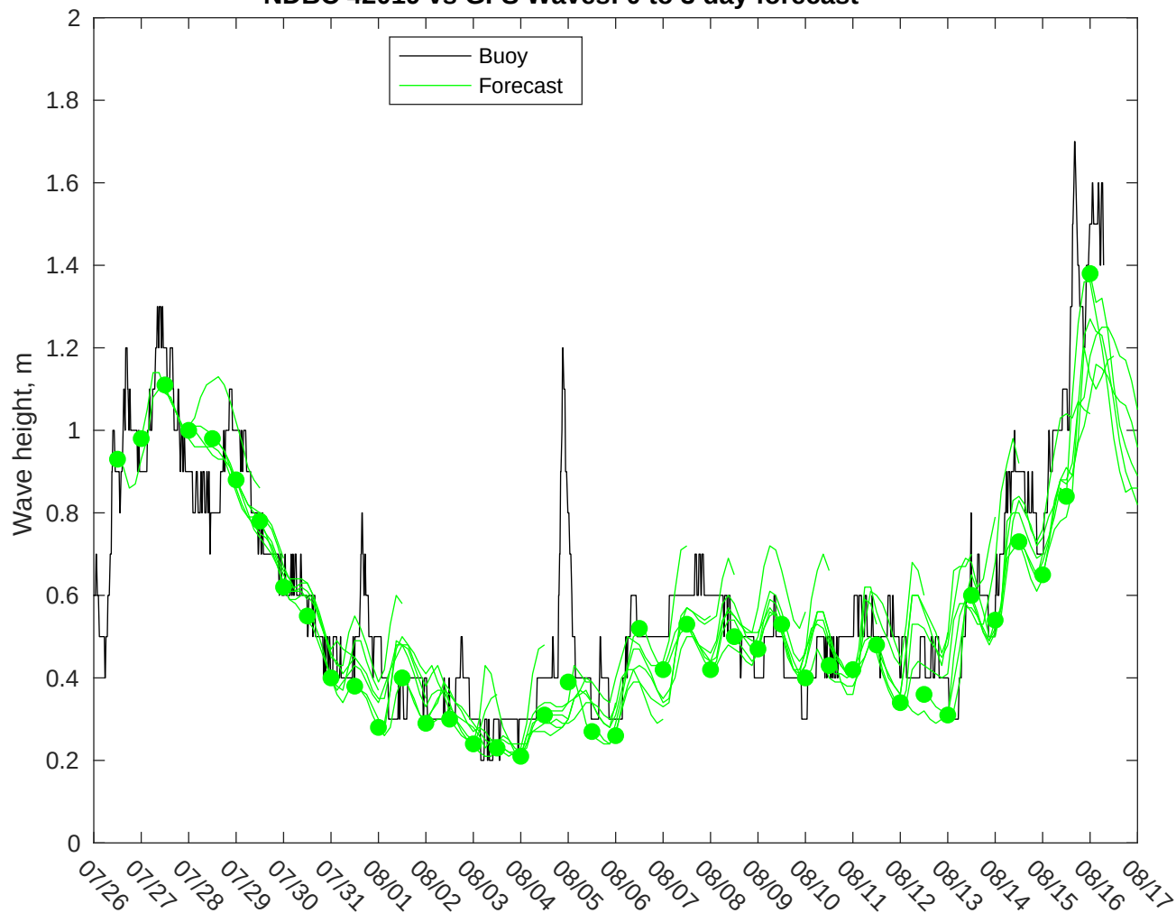
NDBC 42019 vs GFS Waves: 0 to 3 day forecast
