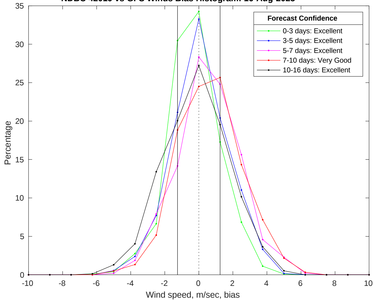
NDBC 42019 vs GFS Winds Bias Histogram: 16-Aug-2025
