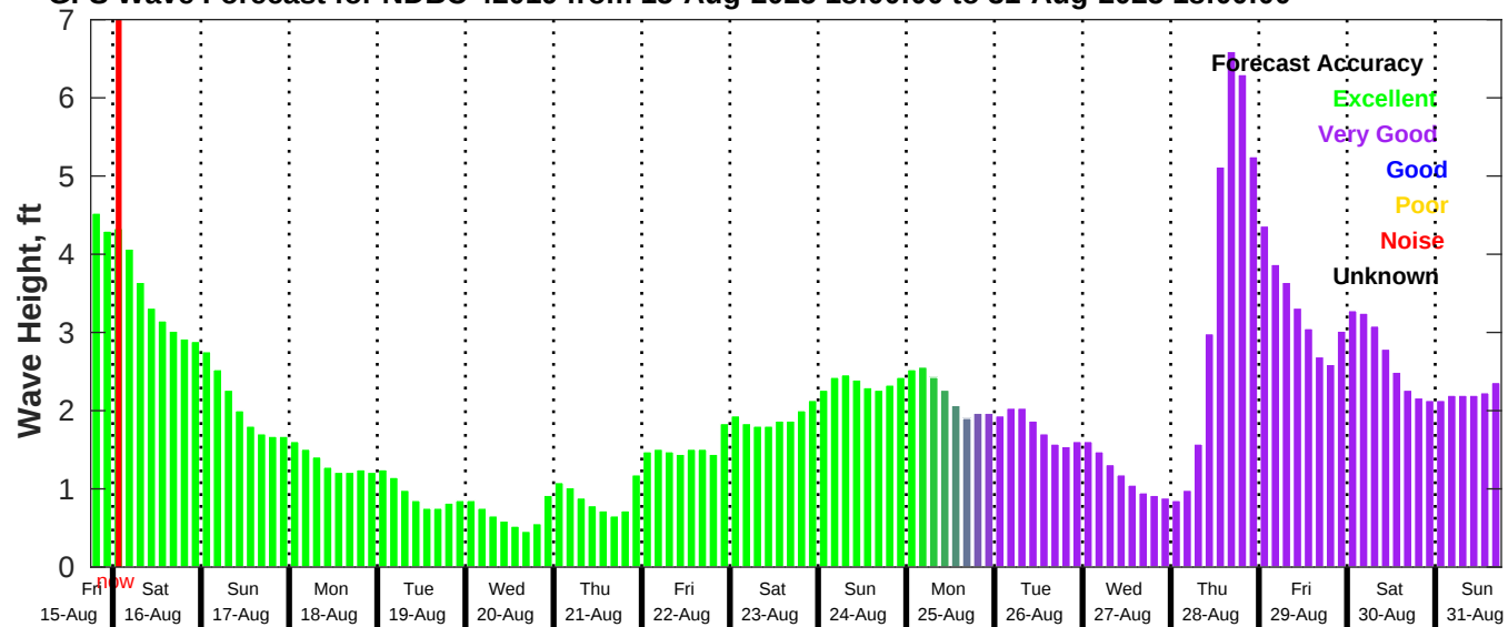
GFS Wave Forecast for NDBC 42019 from 15-Aug-2025 18:00:00 to 31-Aug-2025 18:00:00
