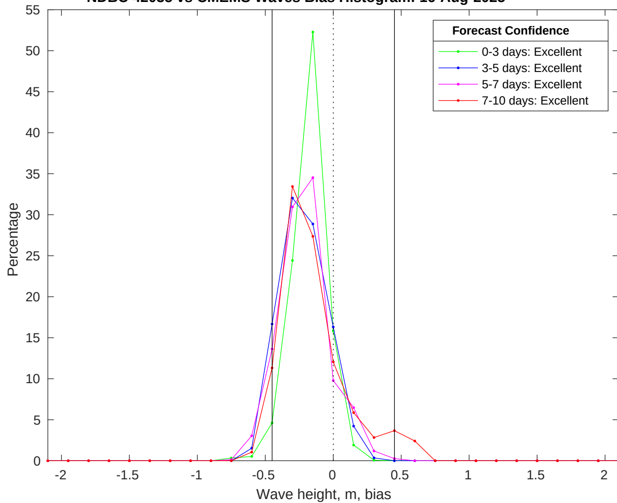
NDBC 42035 vs CMEMS Waves Bias Histogram: 16-Aug-2025
