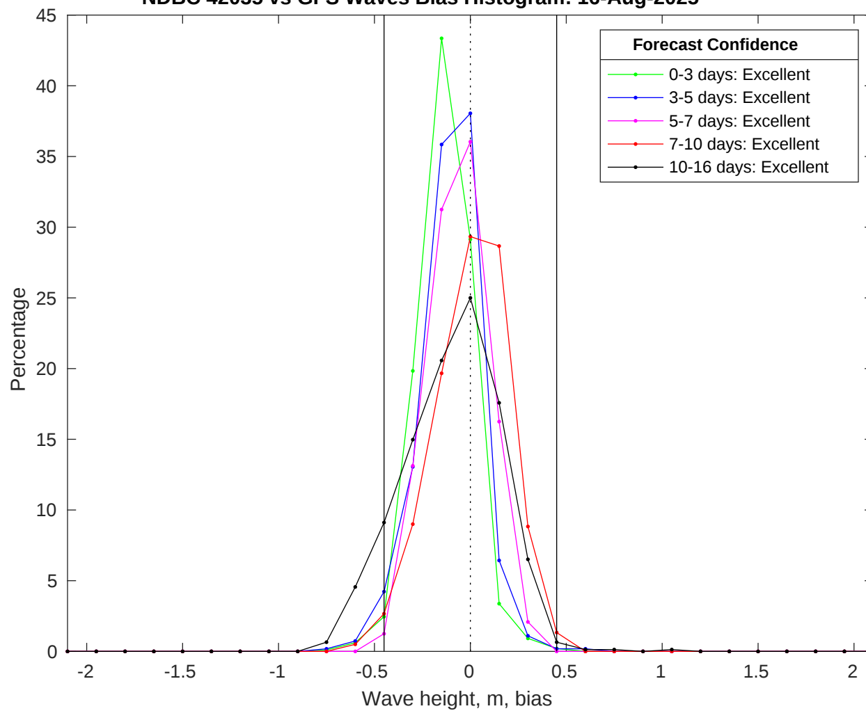
NDBC 42035 vs GFS Waves Bias Histogram: 16-Aug-2025
