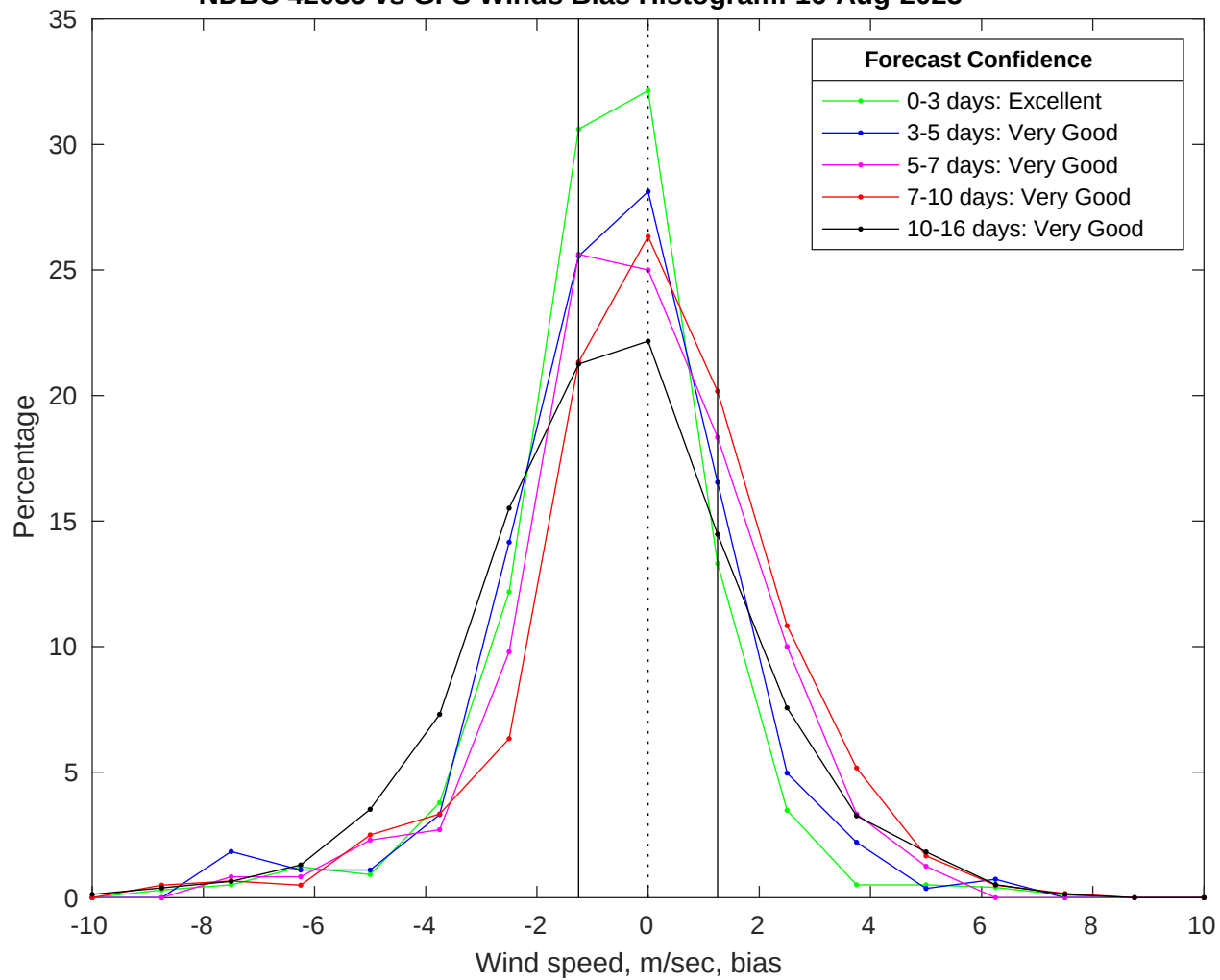
NDBC 42035 vs GFS Winds Bias Histogram: 16-Aug-2025
