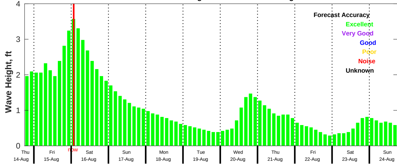
CMEMS Wave Forecast for NDBC 42035 from 14-Aug-2025 18:00:00 to 24-Aug-2025 18:00:00
