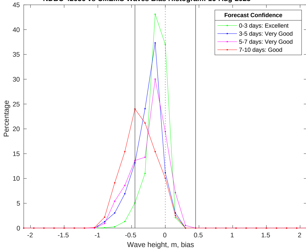
NDBC 42036 vs CMEMS Waves Bias Histogram: 16-Aug-2025
