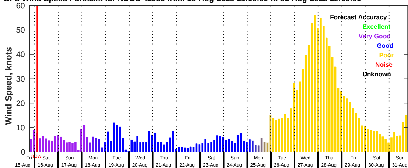
GFS Wind Speed Forecast for NDBC 42036 from 15-Aug-2025 19:00:00 to 31-Aug-2025 19:00:00
