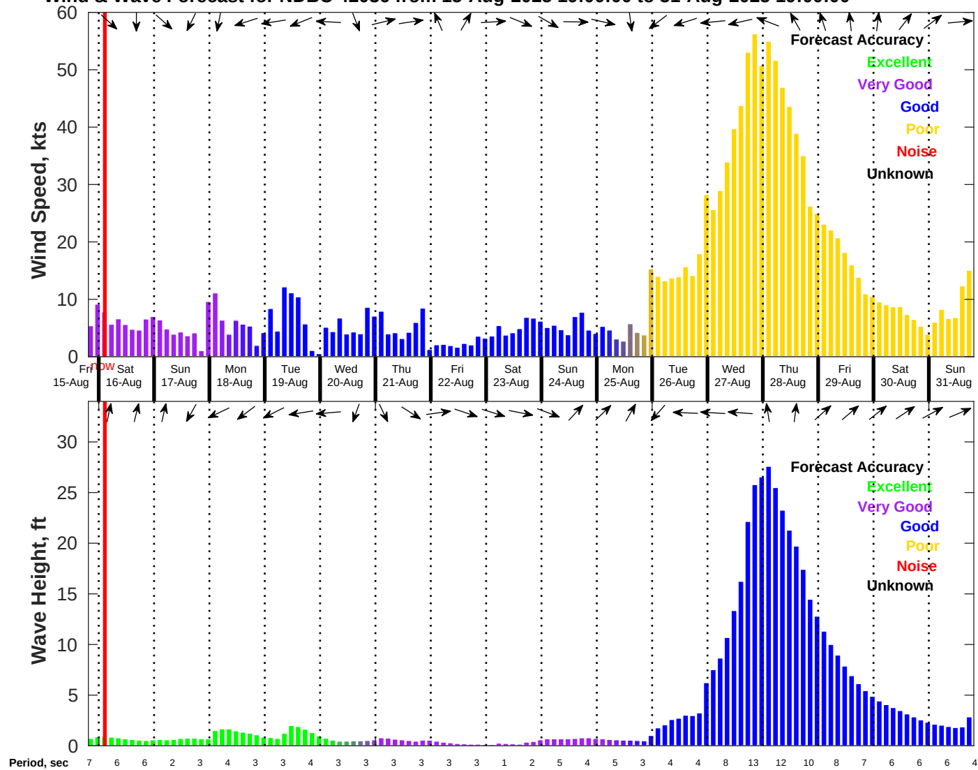
Wind & Wave Forecast for NDBC 42036 from 15-Aug-2025 19:00:00 to 31-Aug-2025 19:00:00
