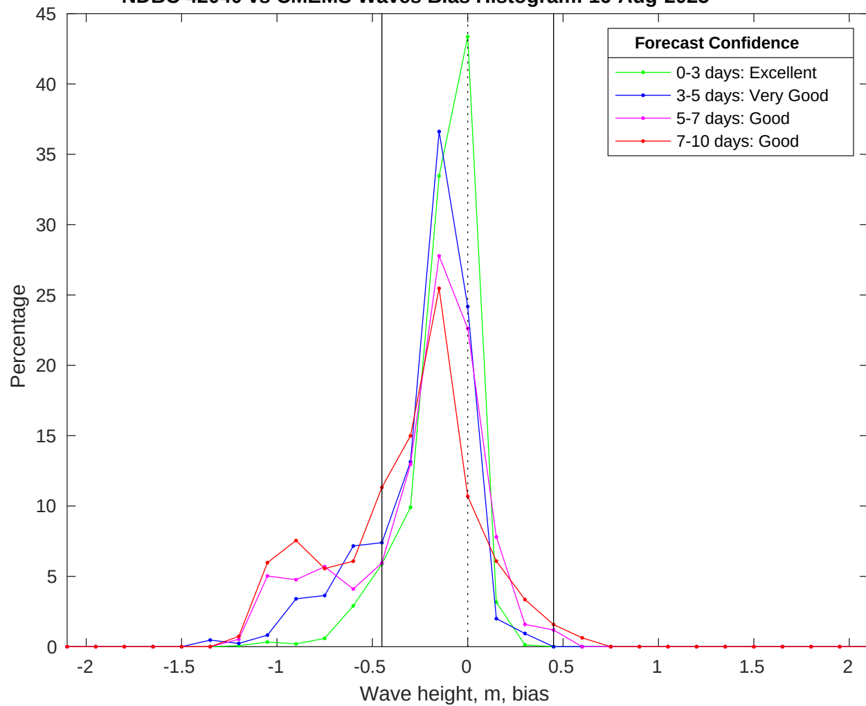
NDBC 42040 vs CMEMS Waves Bias Histogram: 16-Aug-2025
