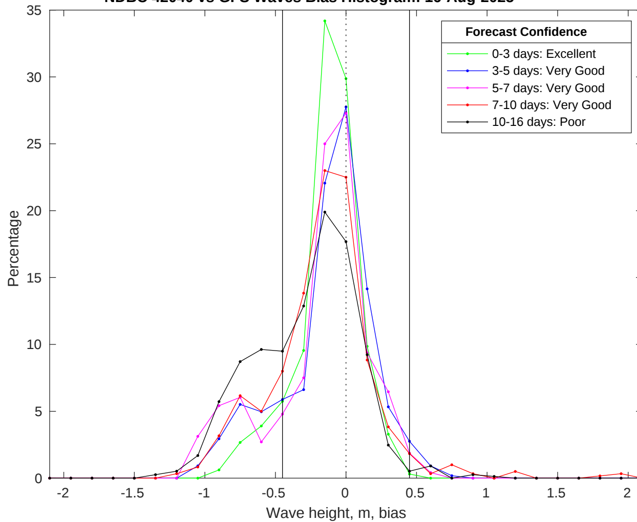
NDBC 42040 vs GFS Waves Bias Histogram: 16-Aug-2025
