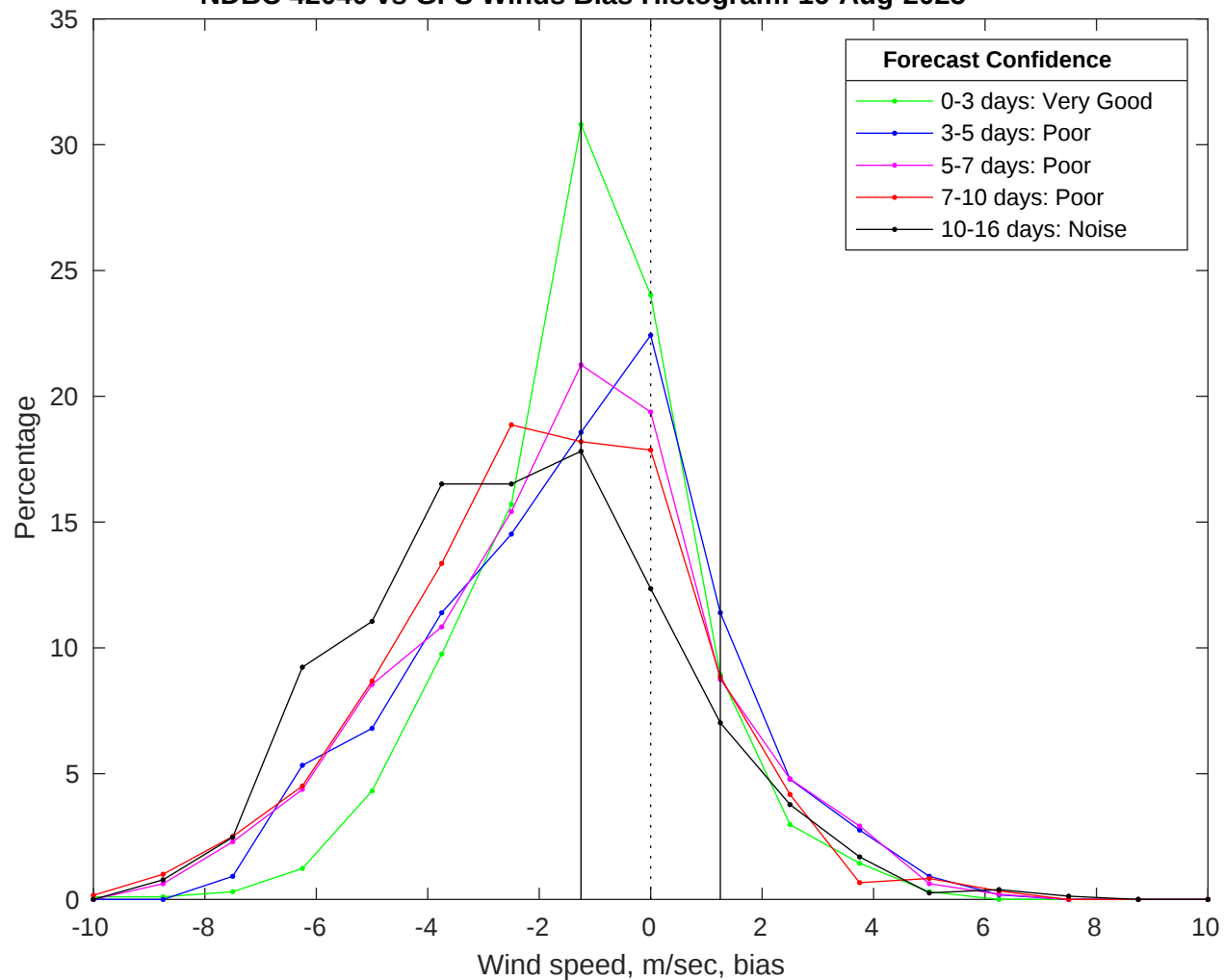
NDBC 42040 vs GFS Winds Bias Histogram: 16-Aug-2025
