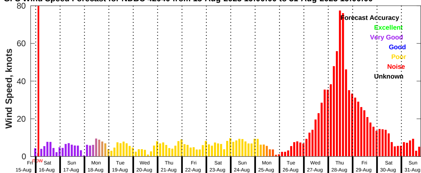
GFS Wind Speed Forecast for NDBC 42040 from 15-Aug-2025 19:00:00 to 31-Aug-2025 19:00:00
