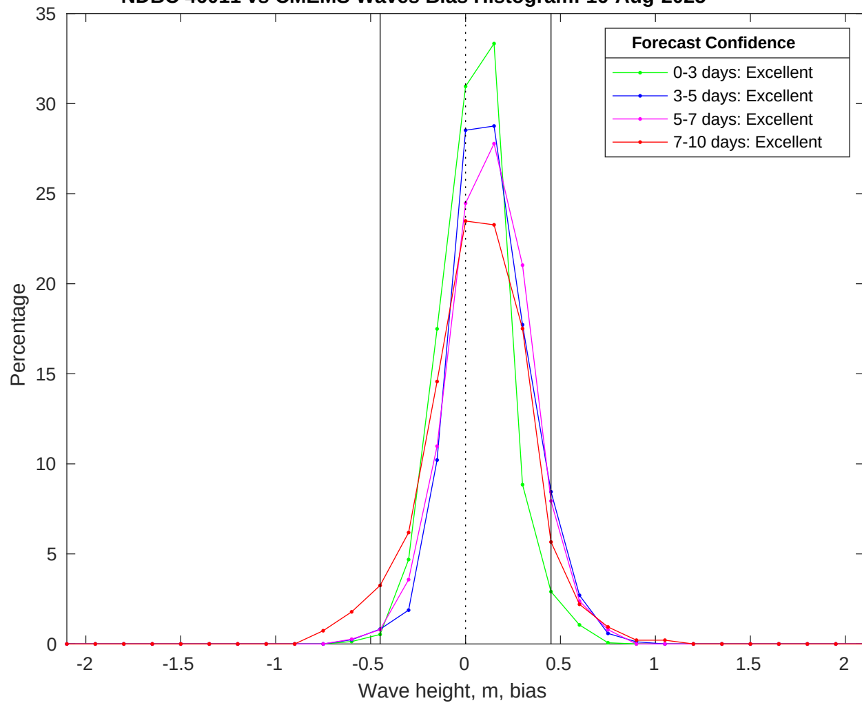
NDBC 46011 vs CMEMS Waves Bias Histogram: 16-Aug-2025
