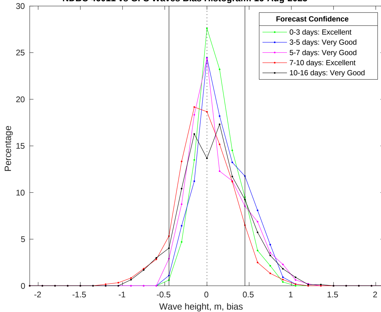
NDBC 46011 vs GFS Waves Bias Histogram: 16-Aug-2025
