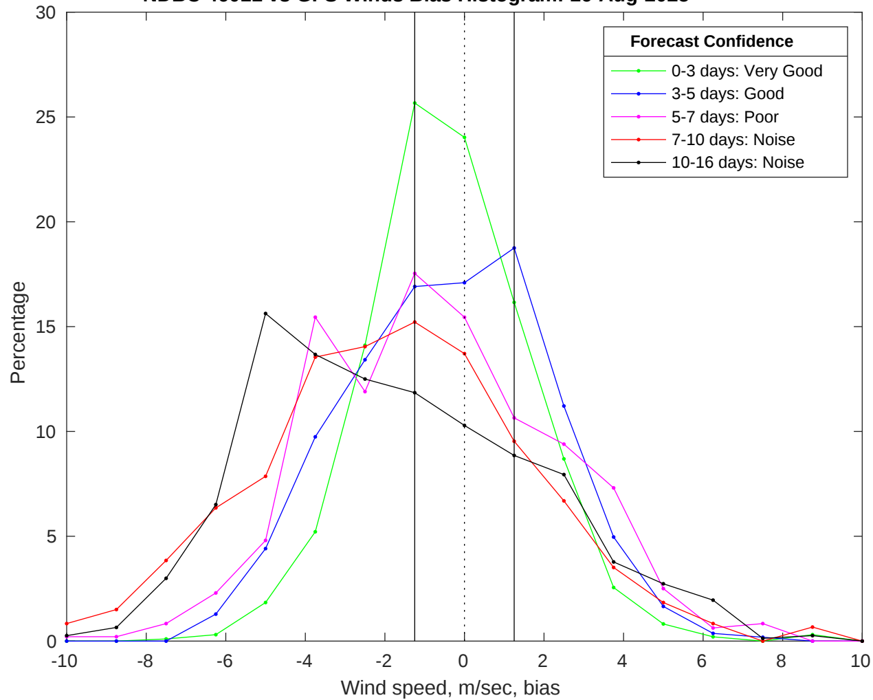
NDBC 46011 vs GFS Winds Bias Histogram: 16-Aug-2025
