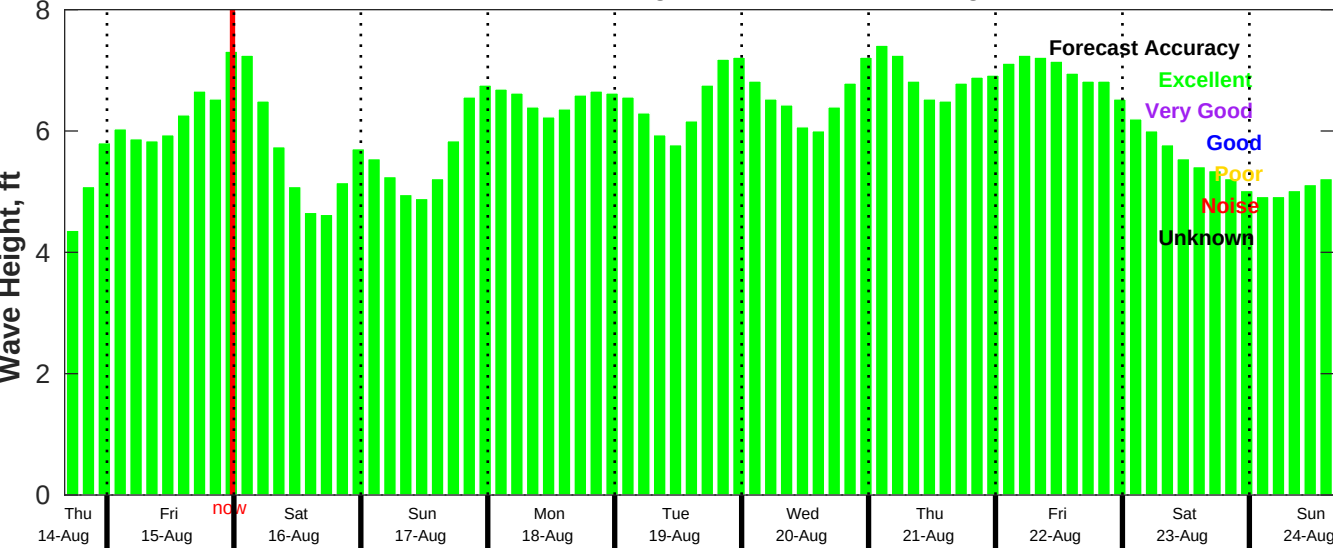
CMEMS Wave Forecast for NDBC 46011 from 14-Aug-2025 16:00:00 to 24-Aug-2025 16:00:00
