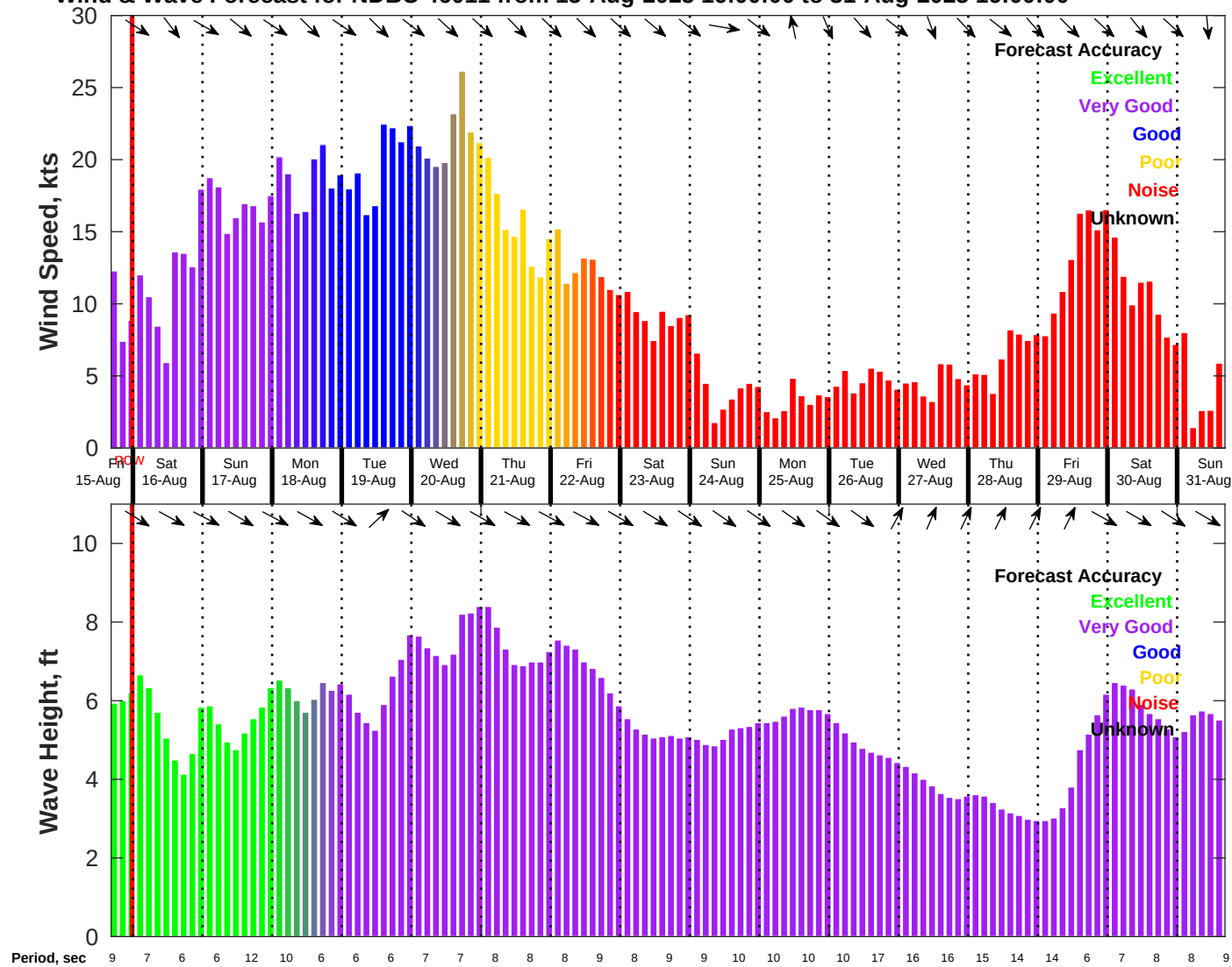
Wind & Wave Forecast for NDBC 46011 from 15-Aug-2025 16:00:00 to 31-Aug-2025 16:00:00
