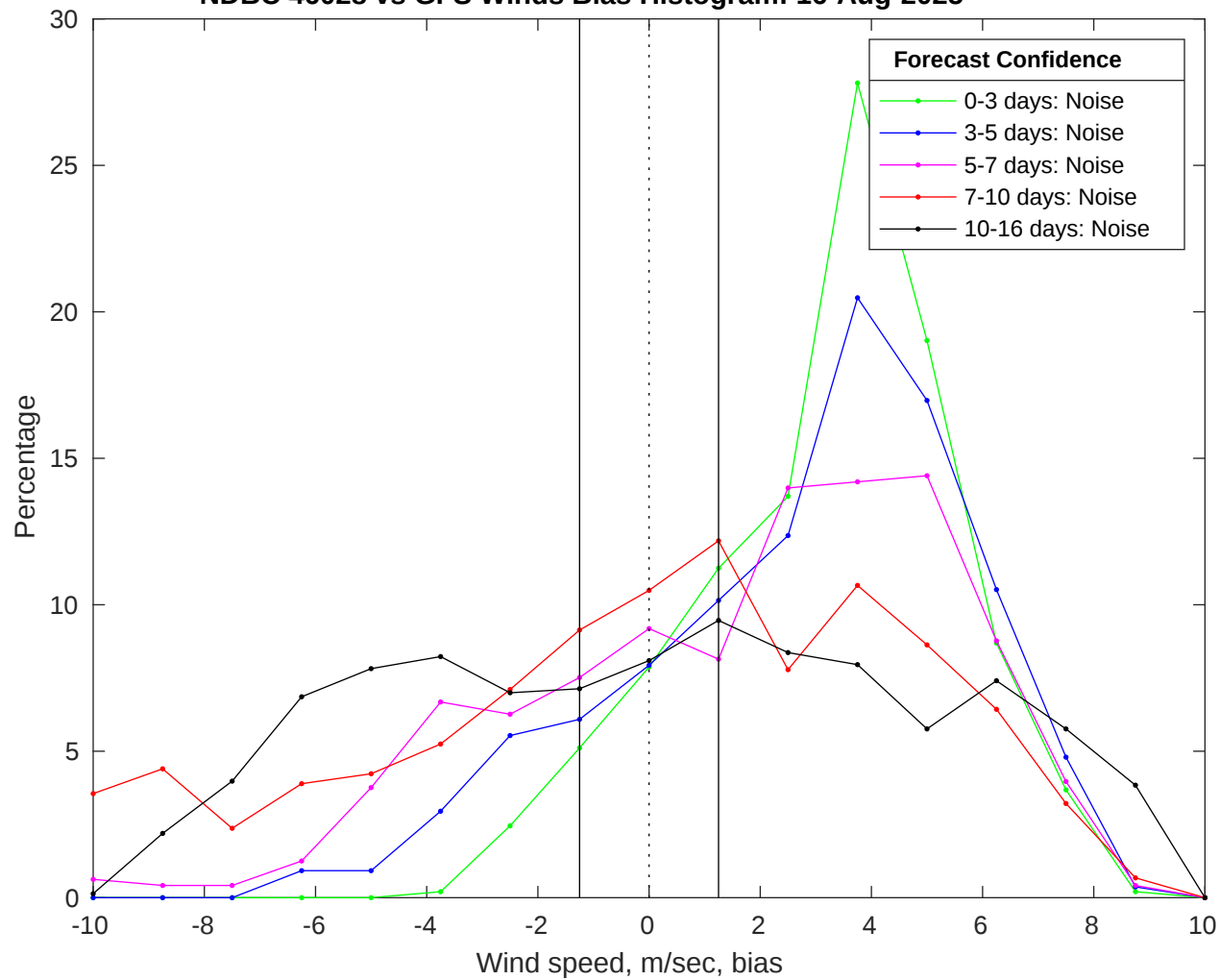
NDBC 46028 vs GFS Winds Bias Histogram: 16-Aug-2025
